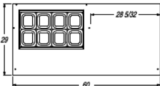
SPE60-08 TOP VIEW
